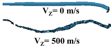
Fig. 5 Deformed shape for different normal velocities of counter plate ( L = 0.6 m, t = 0.05 m, \theta = 30^\circ , V_x = -500 m/s)
