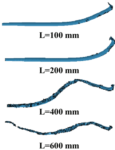
Fig. 4 Deformed shape for various lengths of counter plate ( t = 0.05 m, \theta = 30^\circ , V_x = -500 m/s, V_z = 500 m/s)
