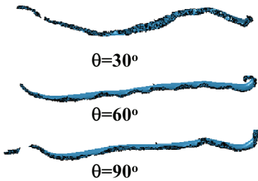
Fig. 6 Deformed shape for various collision angles of projectile with counter plate ( L = 0.6 m, t = 0.05 m, V_x = -500 m/s, V_z = 500 m/s)
