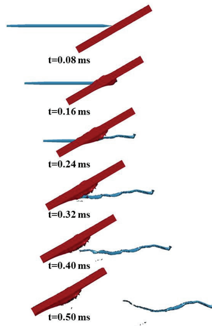
Fig. 2 Penetration procedure of a projectile into a plate (L = 0.6 m, t = 0.05 m, \theta = 30^\circ , V_x = -500 m/s, V_z = 500 m/s)
