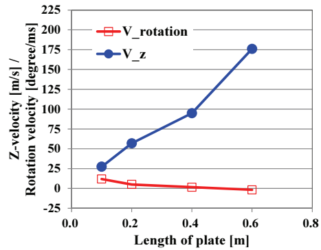
Fig. 7 Z-directional and rotational velocity of projectile for various plate length ( t = 0.05 m, \theta = 30^\circ , V_x = -500 m/s, V_z = 500 m/s)
