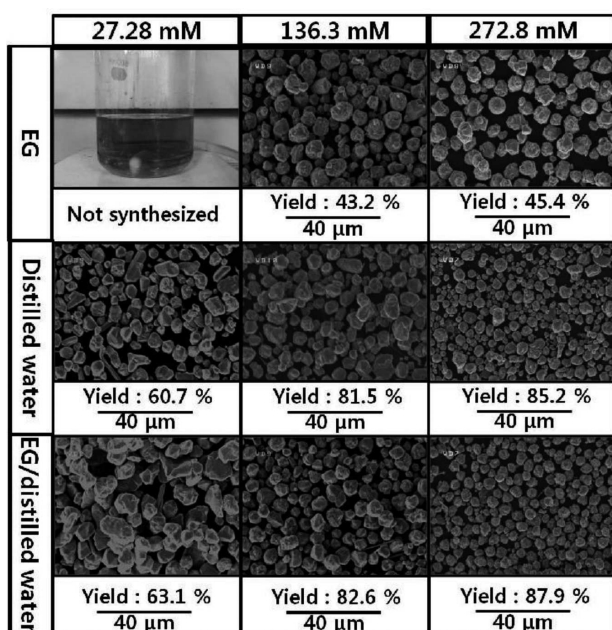
Fig. 5. SEM images and yields of Cu powders synthesized in 3 h at 90°C with different solvent types and amounts of L-ascorbic acid
