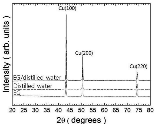
Fig. 3. XRD results of Cu powders synthesized in 3 h at 70°C with different solvent types
