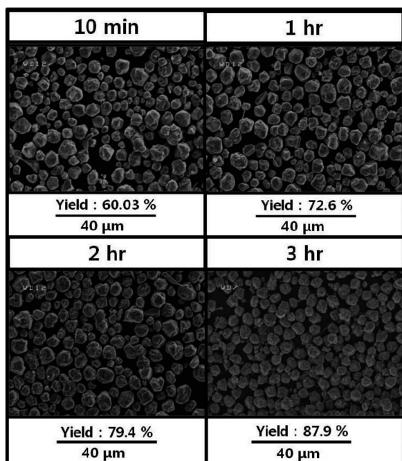
Fig. 7. SEM images and yields of Cu powders synthesized in a mixture solvent of ethylene glycol and distilled water at 90°C with different times (the added amount of L-ascorbic acid was 272.8 mM)
