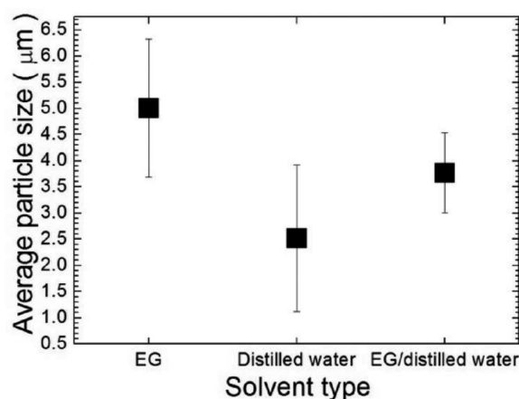
Fig. 6. Size distribution of Cu powders synthesized in 3 h at 90°C with different solvent types (the added amount of L-ascorbic acid was 272.8 mM)
