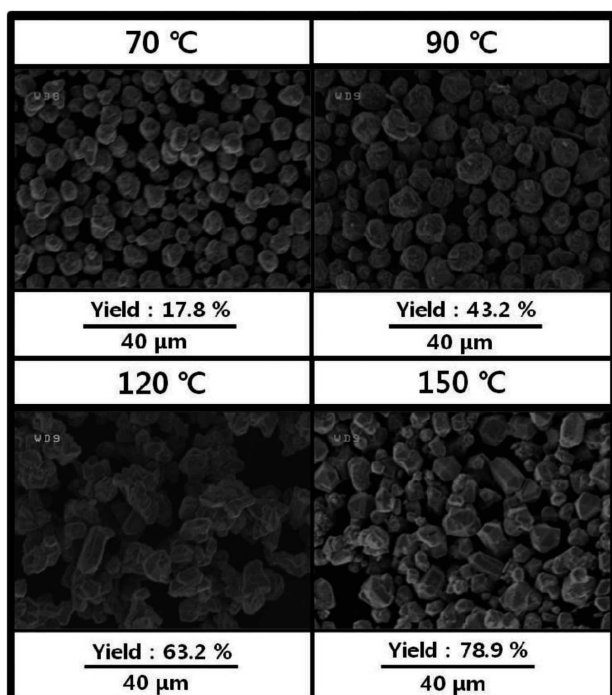
Fig. 4. SEM images and yields of Cu powders synthesized in an ethylene glycol for 3 h at different temperatures
