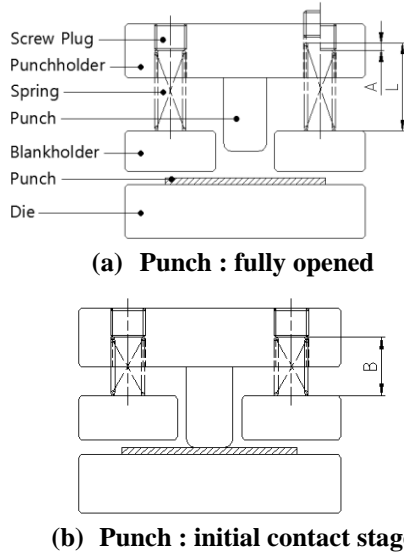
Fig. 2 Determination of blankholding force
