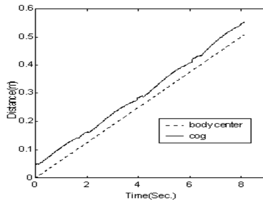
Figure 6. The reference trajectory for the body center and the corresponding trajectory of the total gravity center without the body impedance control
