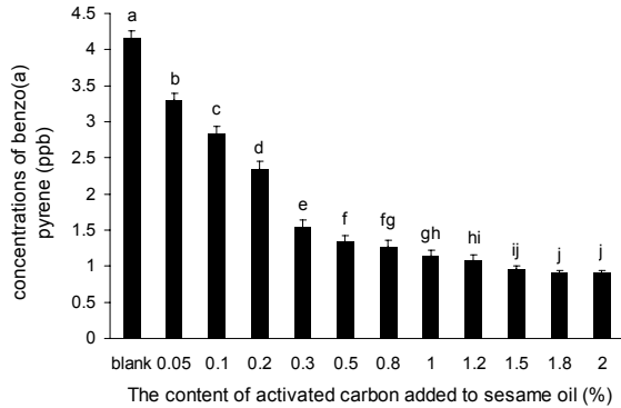
Fig. 4. Reduction of benzo(a)pyrene in sesame oil by addition of active carbon on sesame oil. Those different superscript letters indicate significantly different at P < 0.05 by Duncan's multiple range tests.
