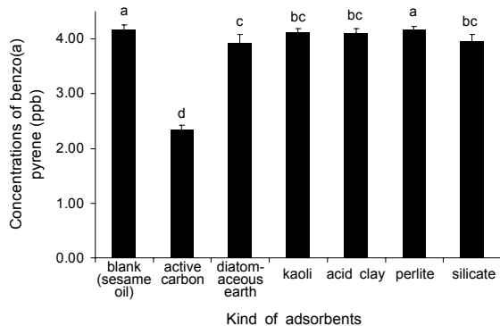
Fig. 3. Effects of adsorbents on the reduction of benzo(a)pyrene in sesame oil. Sesame oil was spiked with 4.1 ppb benzo(a)pyrene and stirred with 0.2% (w/w) adsorbents at 40°C for 15 min. Values are means±SD. Those different superscript letters indicate significantly different at P < 0.05 by Duncan's multiple range tests.
