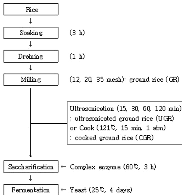
Fig. 1 Schematic diagram of the brewing process of ground rice (GR), cooked ground rice (CGR), and ultrasonicated ground rice (UGR).
