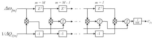
Fig. 6 Discrete-time realization of the cross-correlation function
