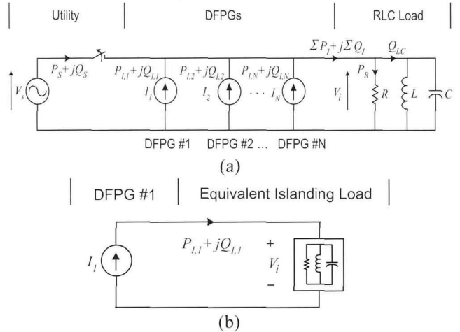
Fig. 2 (a) Full description of an equivalent circuit of islanding, (b) A simplified equivalent circuit of islanding
