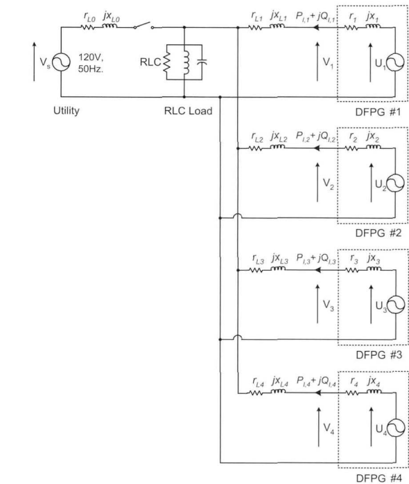
Fig. 8 Simulation circuit
