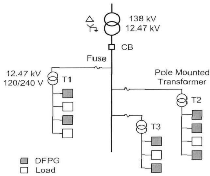
Fig. 1 Multiple DFPGs independently operates in parallel with the utility
