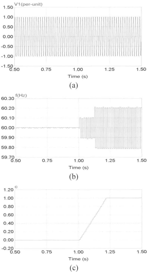
Fig. 9 Simulation results of the proposed method, (a) inverter terminal voltage (per-unit), (b) frequency of the terminal voltage and (c) cross-correlation index C_{[n]}
