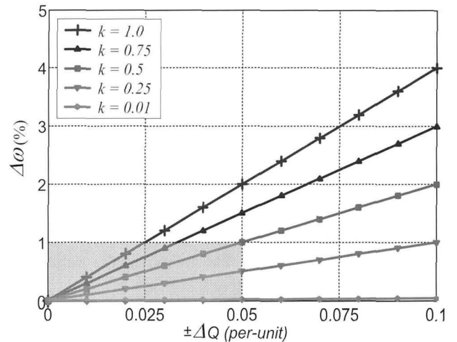
Fig. 3 Frequency deviation versus \Delta Q_{I,i}
