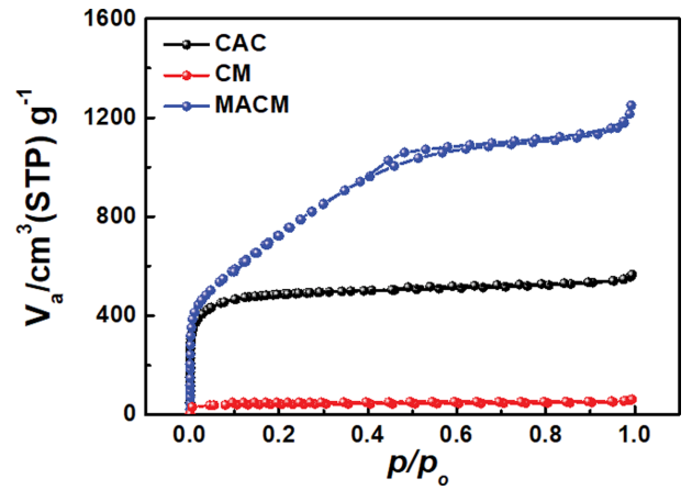
Fig. 4. BET result using N_2 adsorption/desorption of CAC, CM, and MACM.
