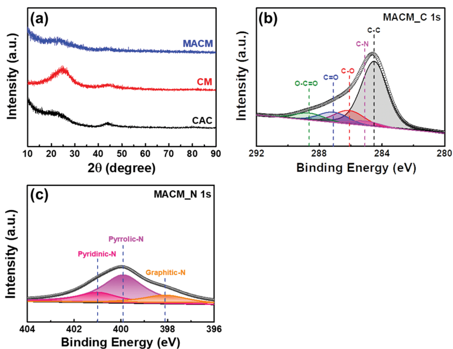
Fig. 3. (a) XRD data of all the samples and (b) XPS spectra of C 1s and N 1s for MACM sample.
