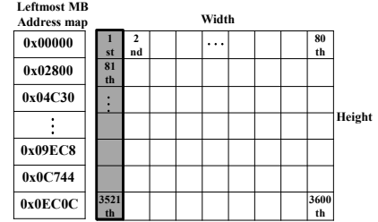
Fig. 5. The leftmost MB address map for an HD frame.
