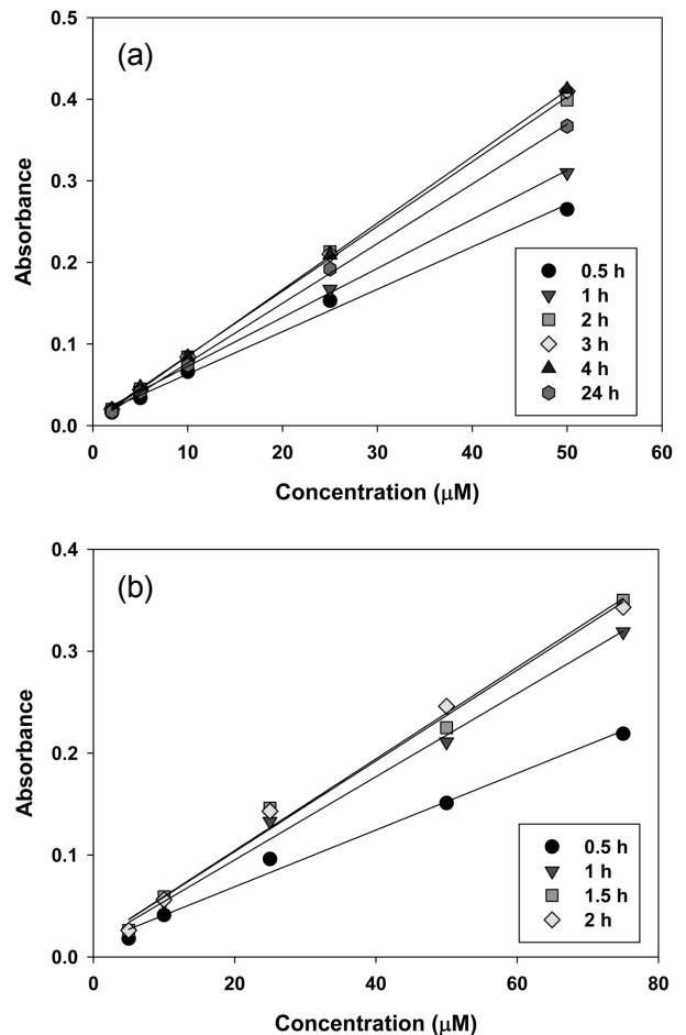
Fig. 3. Standard curves for (a) phenol (0-50 \mu M) and (b) aniline (0-75 \mu M) after reaction with reagent AB ( \text{NH}_2\text{Cl} ) in different reaction time.
