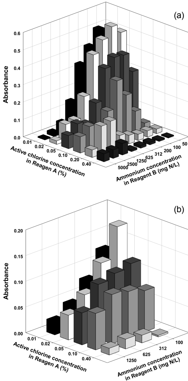
Fig. 2. Optimization of reagent concentration on color development for (a) phenol, and (b) aniline. Note that 50 \mu M of each product was applied, and absorbance was measured after 2 h of reaction.
