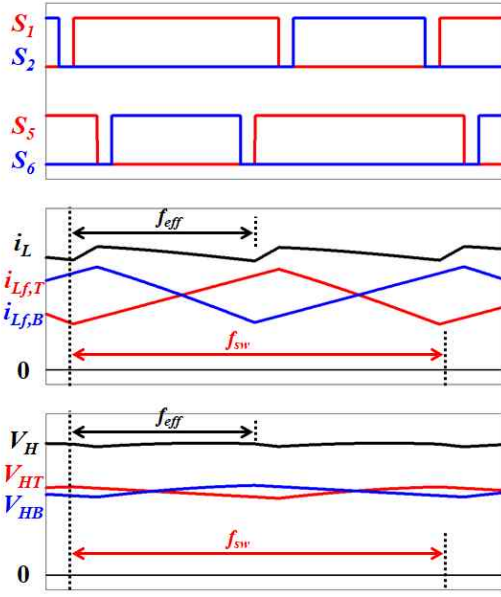
Fig. 6. Simulation waveforms showing interleaving effect of input current( i_L ) and output voltage( V_H ).
