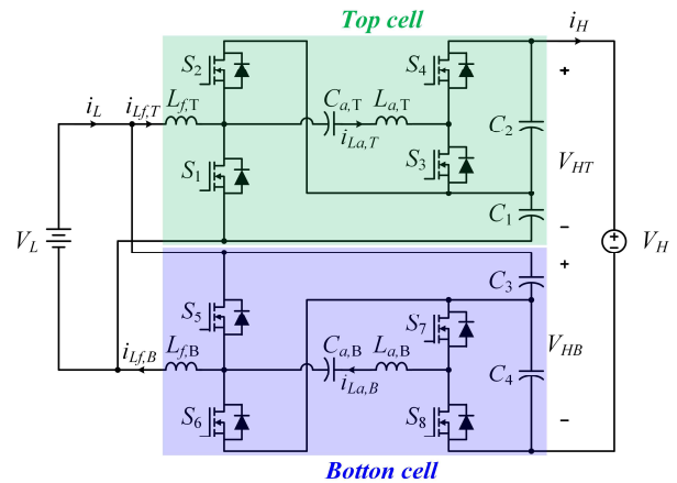
Fig. 2. Proposed non-isolated bidirectional soft-switching DC-DC converter.
