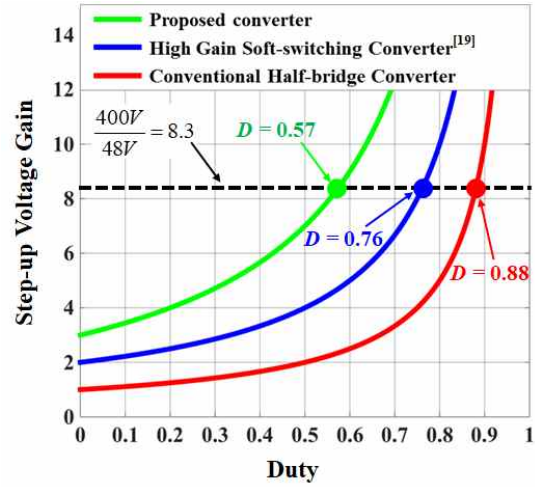
Fig. 5. Ideal voltage gain comparison.
