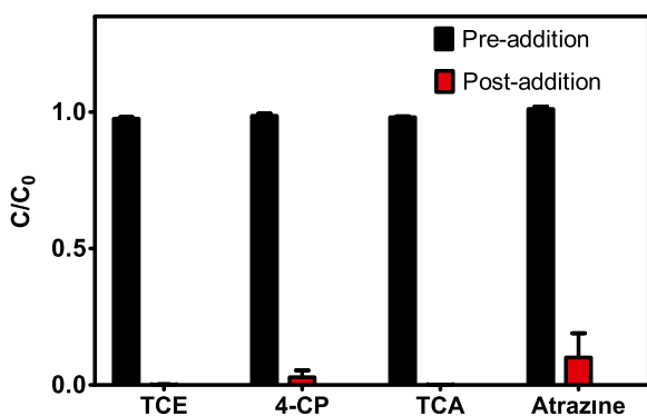
Fig. 4 Effect of nitrate for termination of nZVI's reducing activity ( C_0 , TCE = 300 \mu\text{g/L} , C_0 , 4-CP = 500 \mu\text{M} , C_0 , TCA = 300 \mu\text{g/L} , C_0 , Atrazine = 120 \mu\text{g/L} , C_{\text{Ni/Fe-NPs}} = 2 g/L). Error bars indicate standard deviation based on triplicates
