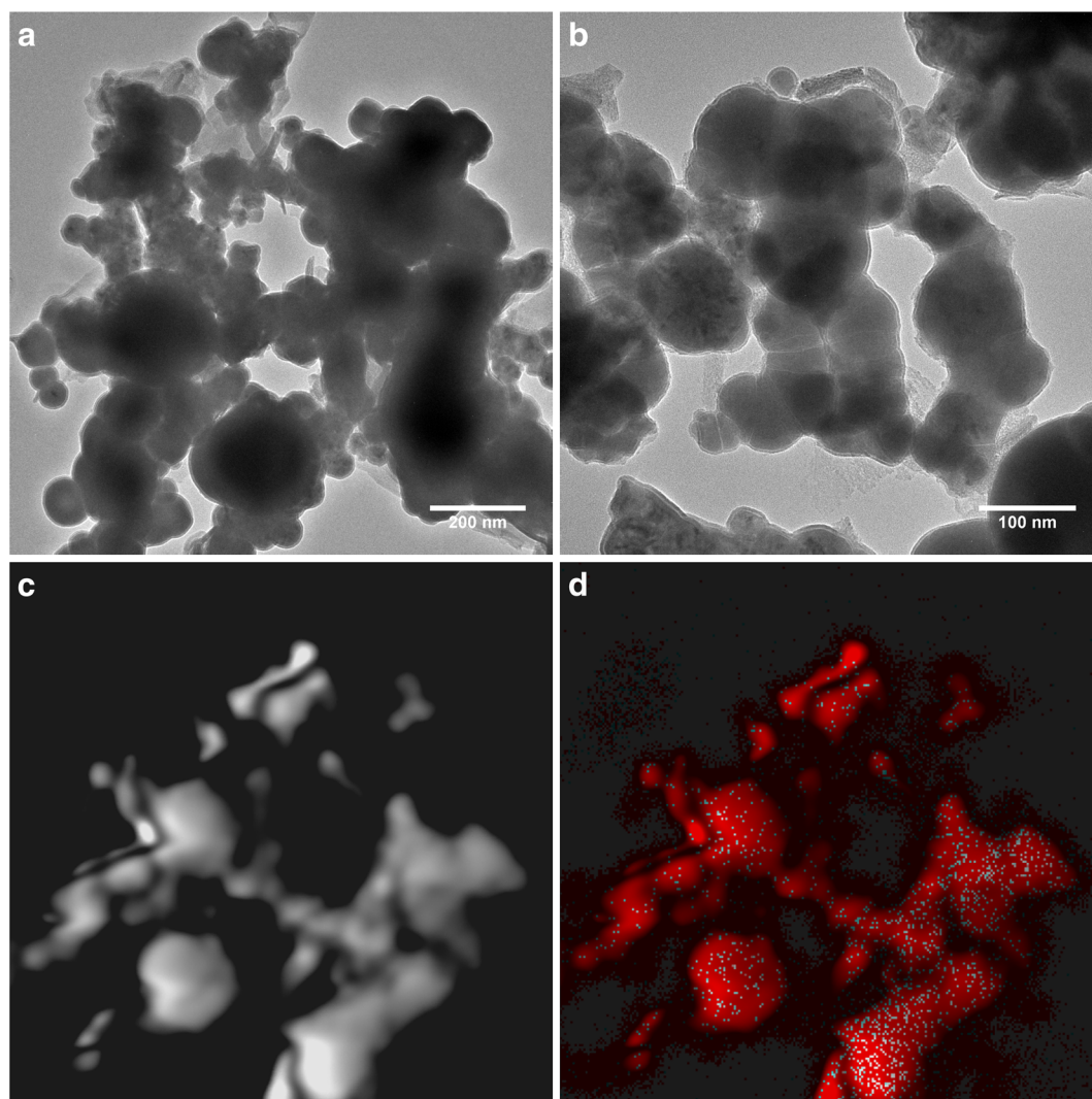
Fig. 1 Electron microscope imaging of Ni/Fe-NPs: a TEM at lower magnification; b TEM at higher magnification; c STEM of image in a ; and d STEM-EDS mapping of image in a with iron
