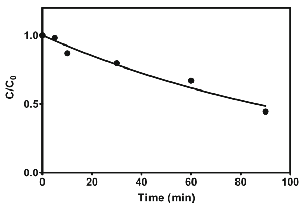
Fig. 5 TCE reduction kinetics obtained by the suggested bromate addition method for reaction termination ( C_0 , TCE = 300 \mu\text{g/L} , C_{\text{Ni/Fe-NPs}} (0.2%-Ni) = 2 g/L)
