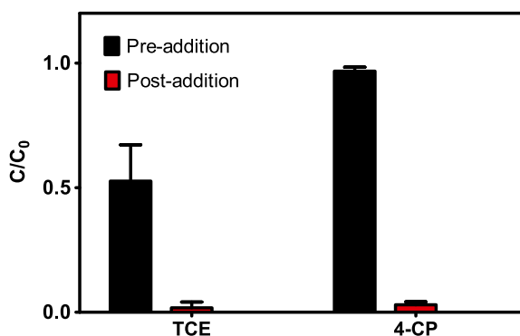
Fig. 3 Effect of nitrate for termination of nZVI's reducing activity ( C_{0, \text{TCE}} = 300 \mu\text{g/L} , C_{0, 4\text{-CP}} = 500 \mu\text{M} , C_{\text{Ni/Fe-NPs}} = 2 \text{ g/L} ). Error bars indicate standard deviation based on triplicates
