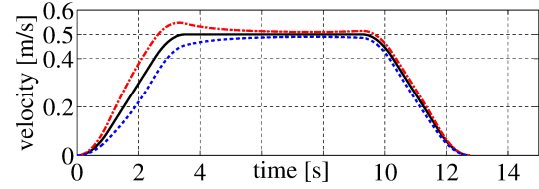
(a) Convolution-based.
