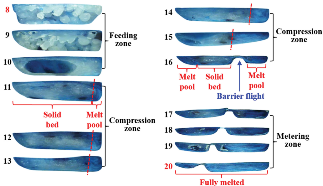
Figure 12. Material distributions in the cross channel sections of closed type barrier screw at 30 RPM.
