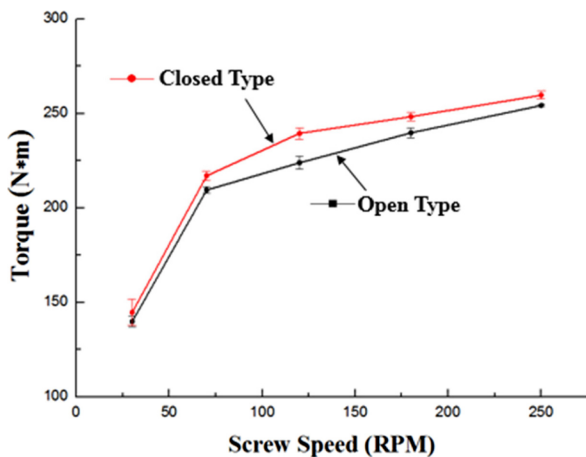
Figure 6. Torque for screw RPM.
