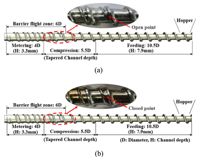
Figure 1. Geometry of barrier screw (a) open type; (b) closed type.
