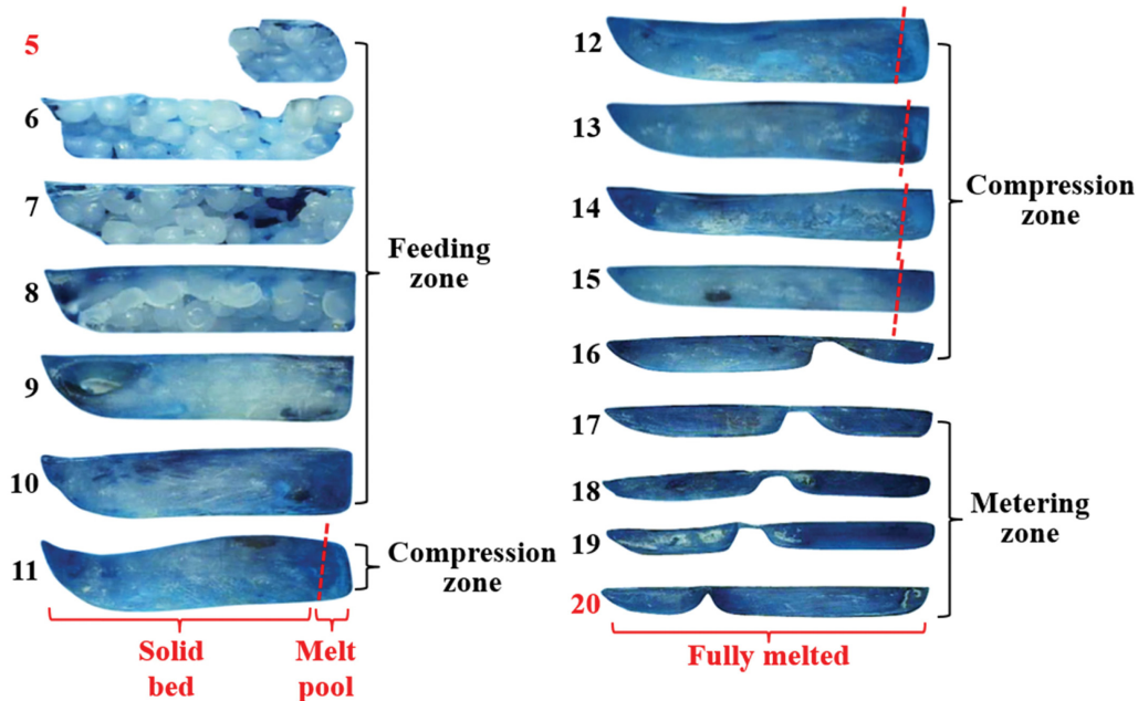
Figure 13. Material distributions in the cross channel sections of closed type barrier screw at 180 RPM.
