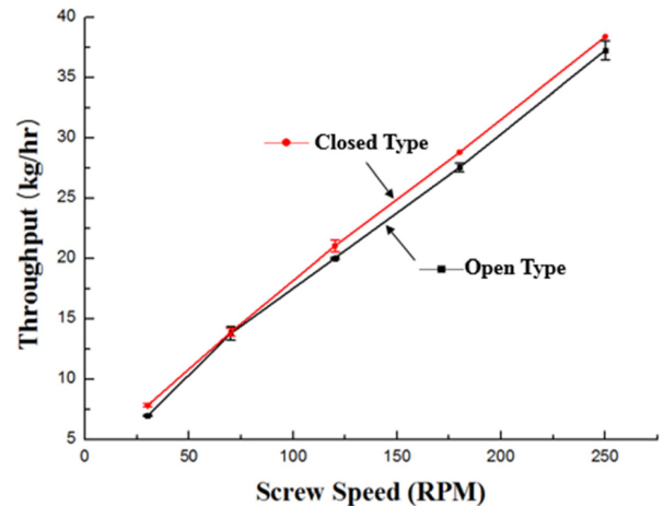
Figure 4. Variation of throughput with screw RPM.
