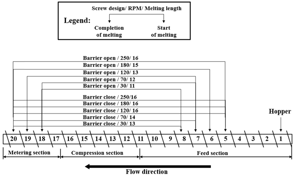
Figure 15. Locations of start of melting and completion of melting in barrier screw.
