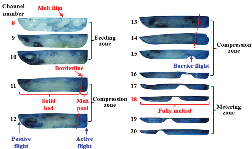
Figure 10. Material distributions in the cross channel sections of open type barrier screw at 30 RPM.
