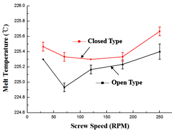
Figure 7. Melt temperature for screw RPM.
