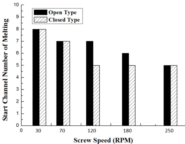
Figure 16. Starting channel number of melting in barrier screw according to screw RPM.
