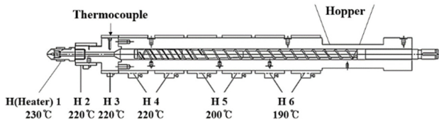
Figure 3. Locations of temperature sensors and barrel temperature settings.
