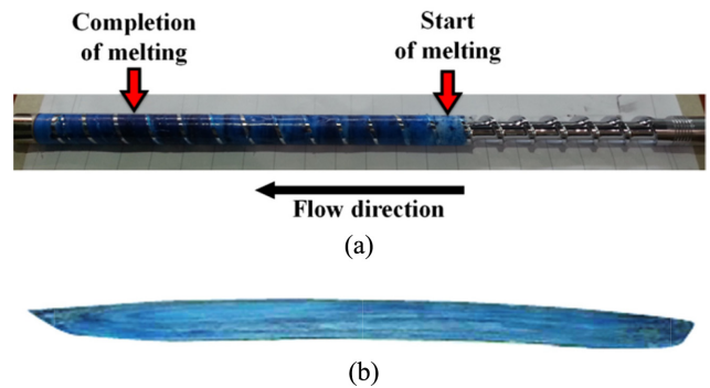
Figure 8. Start and completion locations of melting (a) material distribution in a screw; (b) completed melted material in the cross section of screw.
