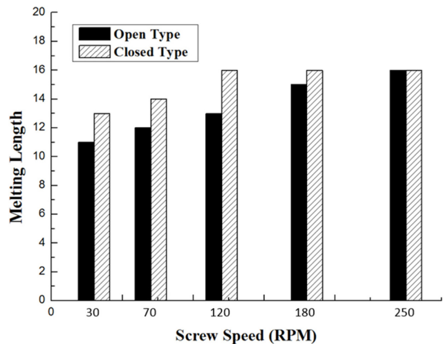
Figure 17. Melting length in barrier screw according to screw RPM.
