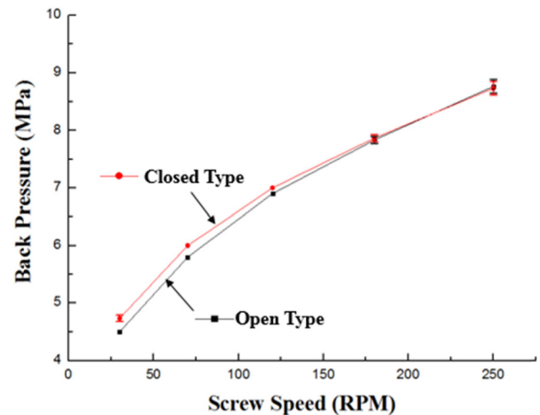
Figure 5. Variation of back pressure with screw RPM.
