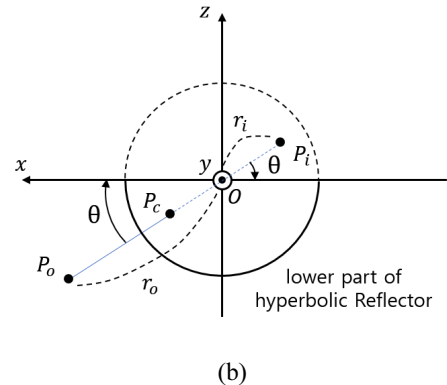
FIG. 4. Image acquisition model for lower part of the mirror: (a) Cross-section in x-y(r-y) plane, (b) Front view.
