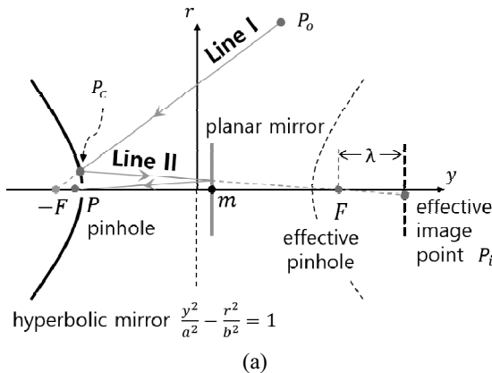
FIG. 4. Image acquisition model for lower part of the mirror: (a) Cross-section in x-y(r-y) plane, (b) Front view.
