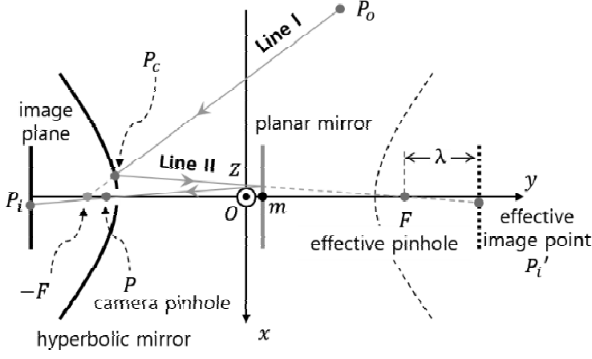
FIG. 3. Image acquisition model on horizontal plane.
