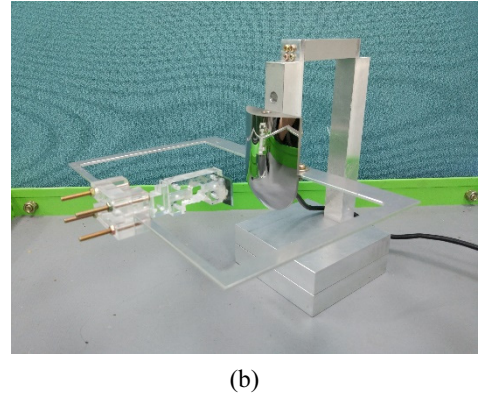
FIG. 8. Imaging system using a combined hyperbolic mirror and secondary planar mirror: (a) Front and rear view of combined hyperbolic mirror with a camera, (b) Experimental setup with the secondary planar mirror.
