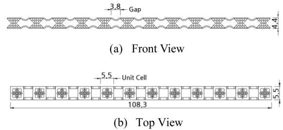
Figure 3. Strip of Pyramidal Kagome Core.
