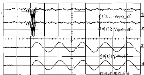
(10msec/div 컨버터1, 2 Vqse_ref 200V/div 컨버터1, 2 입력전류 100A/div)
