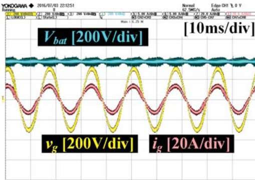
(b) v_g , i_g and V_{bat}
