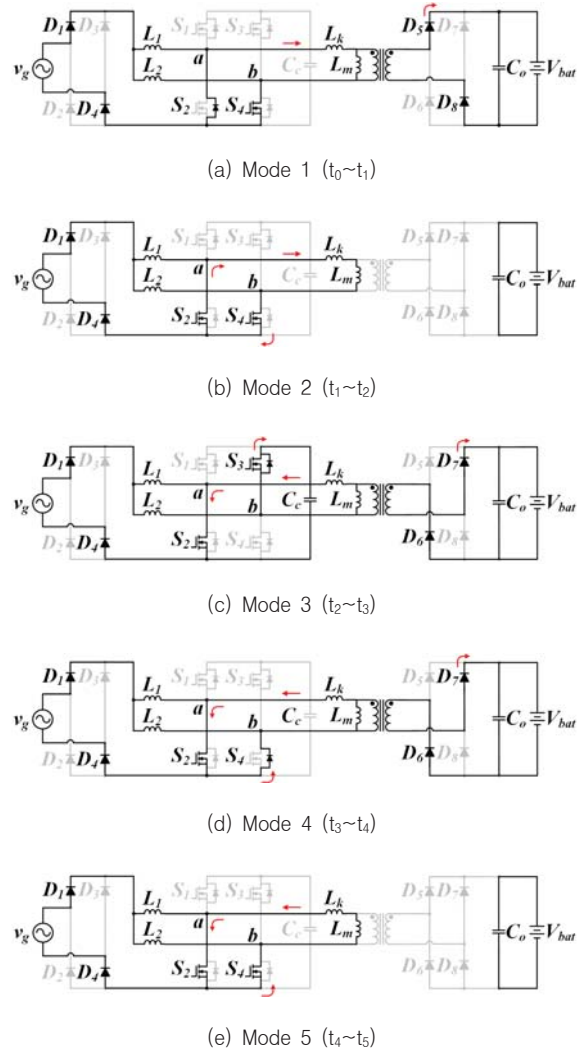
Fig. 3. Operation states of the proposed EV charger.
