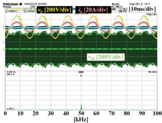
(c) Waveform and FFT of transformer
