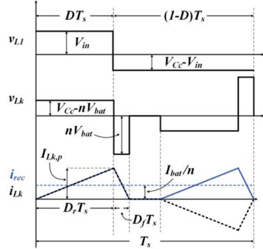
Fig. 7. Inductor voltage waveforms of the leakage and input inductor and current waveforms of the leakage inductor and secondary rectifier.
