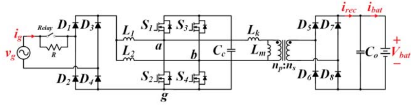
Fig. 1. Proposed single-stage interleaved electrolytic capacitor-less EV charger.
