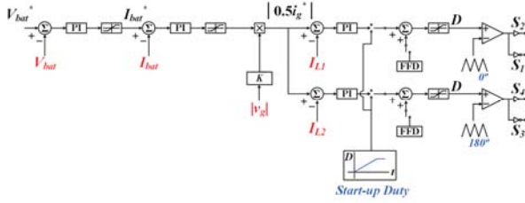
Fig. 5. Control algorithm of the proposed EV charger.
