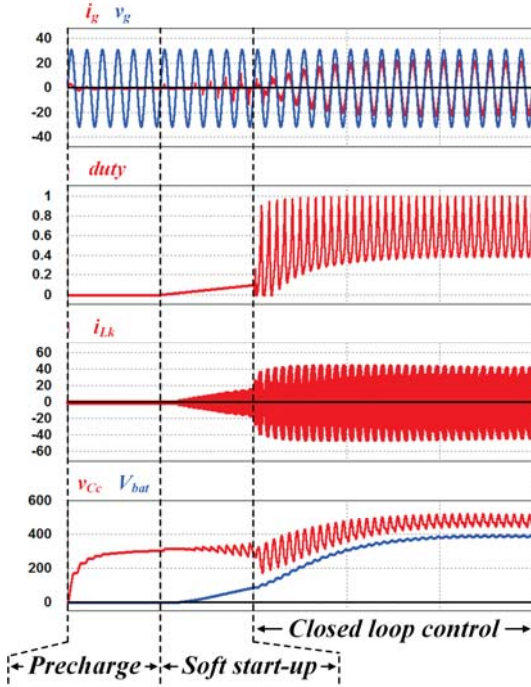
Fig. 6. Start-up operating waveform of the proposed EV charger.
