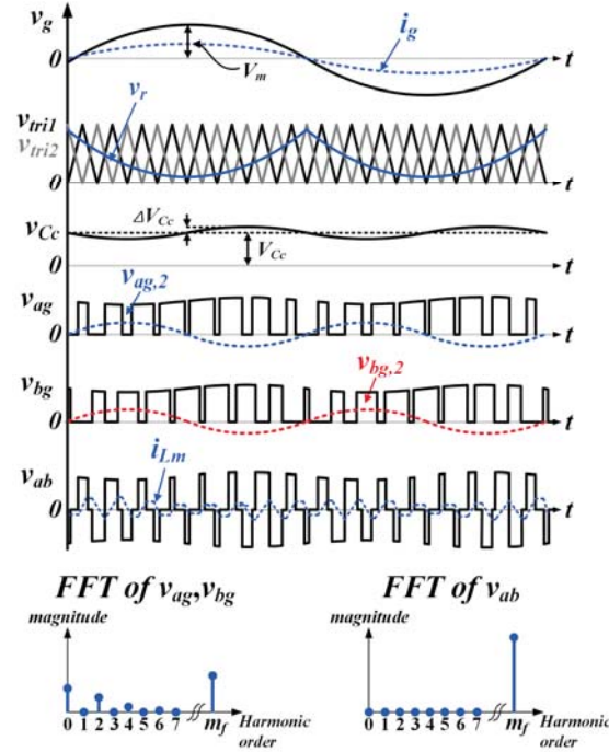
Fig. 4. Key waveform and FFT of the proposed EV charger.
