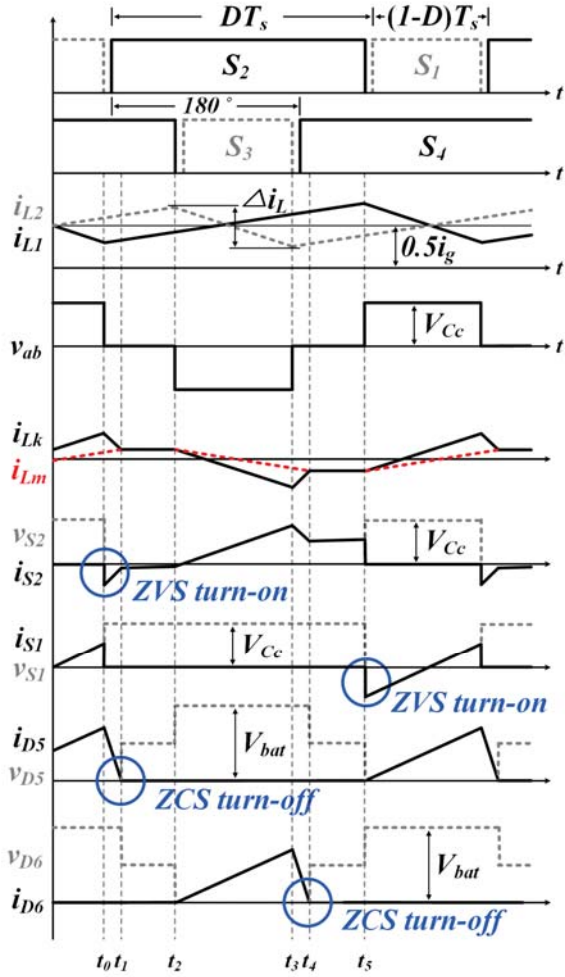
Fig. 2. Operational waveform of the proposed EV charger.
