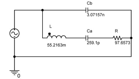
(a) 등가회로 모델 (a) Equivalent circuit model
