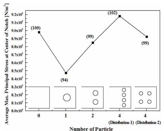
Figure 10. Comparison of average maximum principal stress at the center of notch surface according to total surface area of rubber particle and particle distribution while the total volume of rubber particle is fixed.
