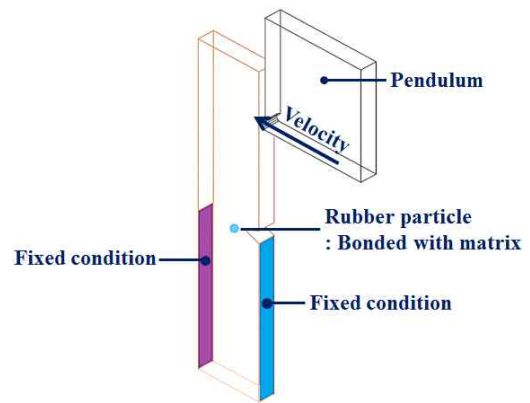
Figure 3. Boundary conditions for computer simulation of Izod impact test.
