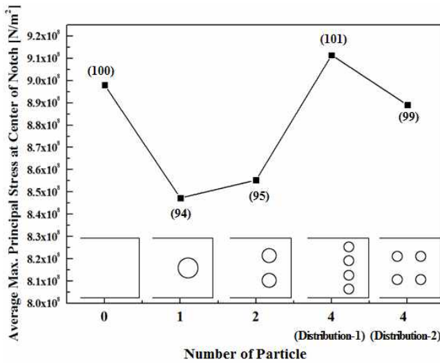
Figure 7. Comparison of average maximum principal stress at the center of notch surface according to number of rubber particle and particle distribution while the surface area of rubber particle is fixed.
